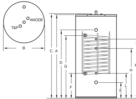
LS-RTV-120-L (Floor to Top Spare 3/4" NPT Tank Connection is 42 3 / 4 "") (Floor to Bottom Spare 3/4" NPT Tank Connection is 17 7 / 8 "")
